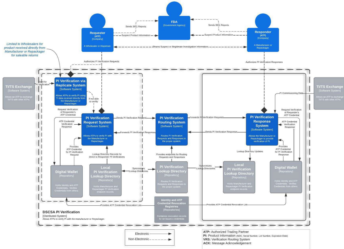
Figure 1 – PI Verification Request is routed to another VRS solution using the LD connectivity information.
